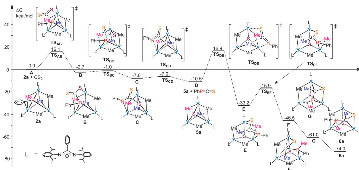
Figure 3. Computed energy profile (Gibbs free energies in kcal mol −1 ) for the formation of 6a by the reaction of 2a with CS 2 at the M06 L/SDD&6-31G**//ONIOM(TPSS/TPSS/LanL2DZ&6-31G**):HF/LanL2 MB level of theory.
